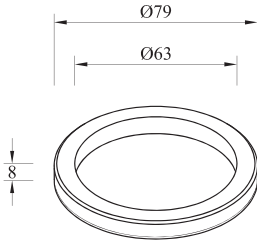
4PR.61 / 4PRSS.61 Reducer Ring Brass and Stainless Steel
