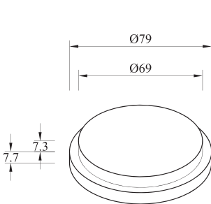
2RH.36 Blanking Cap Teak
