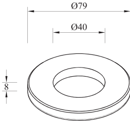
4PR.38 / 4PRSS.38 Reducer Ring Brass and Stainless Steel
