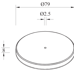
F-APC-/.01/.02/.04 Blanking Cap for Cayman Tables
