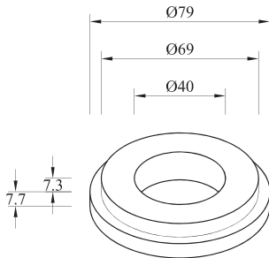
2RH.37 Reducer Ring Teak
